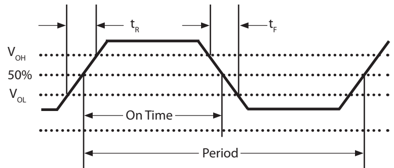
Fig 2: Waveform
