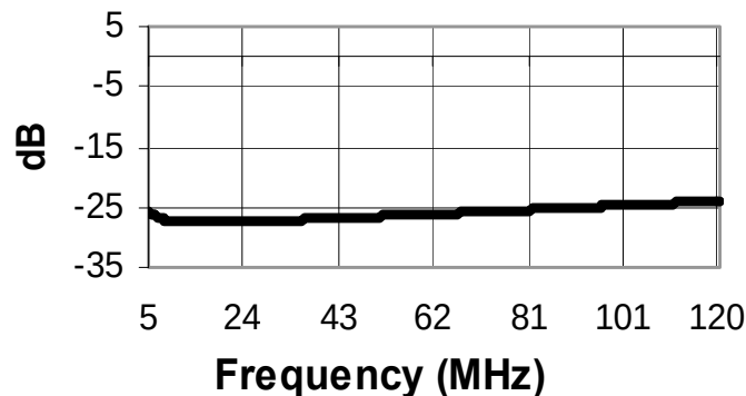
Coupling Return Loss
