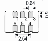
Underside View
