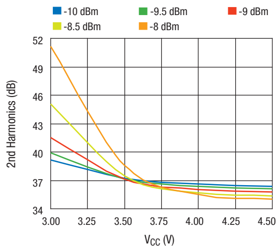
2nd Harmonics vs. V_{CC} Across P_{IN}
