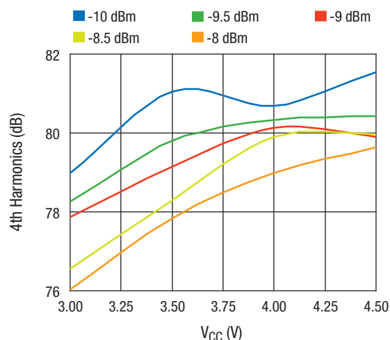
4th Harmonics vs. V_{CC} Across P_{IN}
