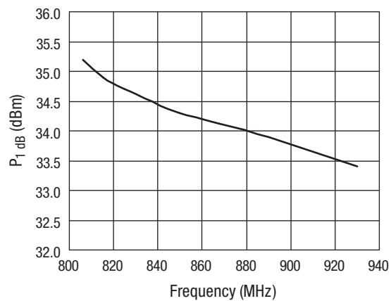
P_{1\text{ dB}} vs. Frequency
