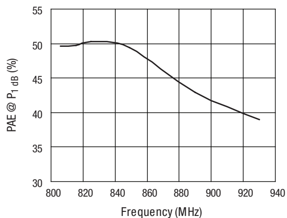
PAE @ P_{1\text{ dB}} vs. Frequency
