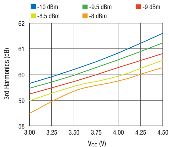
3rd Harmonics vs. V_{CC} Across P_{IN}
