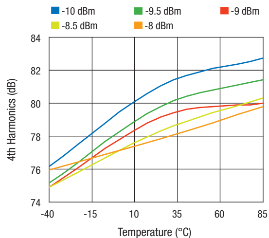
4th Harmonics vs. Temperature Across P_{IN}
