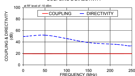
ZMDC-20-3+ COUPLING & DIRECTIVITY
