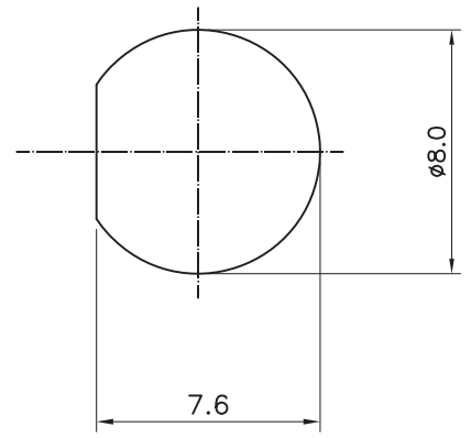
MOUNT HOLES
