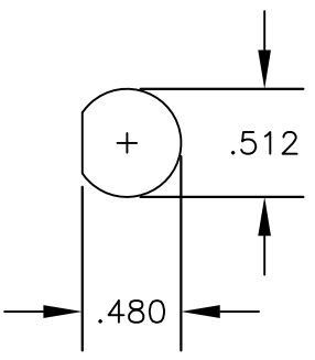
MOUNTING HOLE
