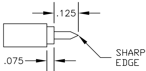
STRIPPING DIMENSIONS
