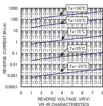
V R -I R CHARACTERISTICS
