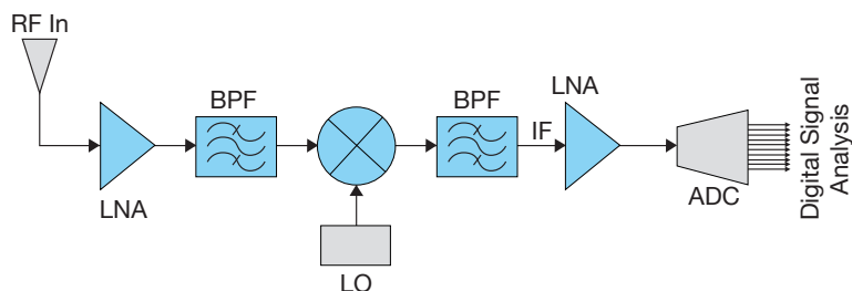
Digital Receiver
