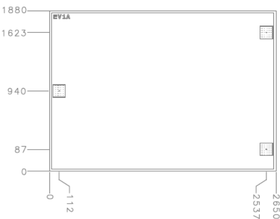
Fig 3. Bonding Pad Positions
