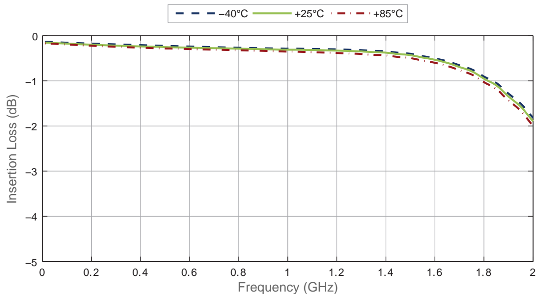
Figure 2 • Insertion Loss vs. Temperature (RFC–RFX)
