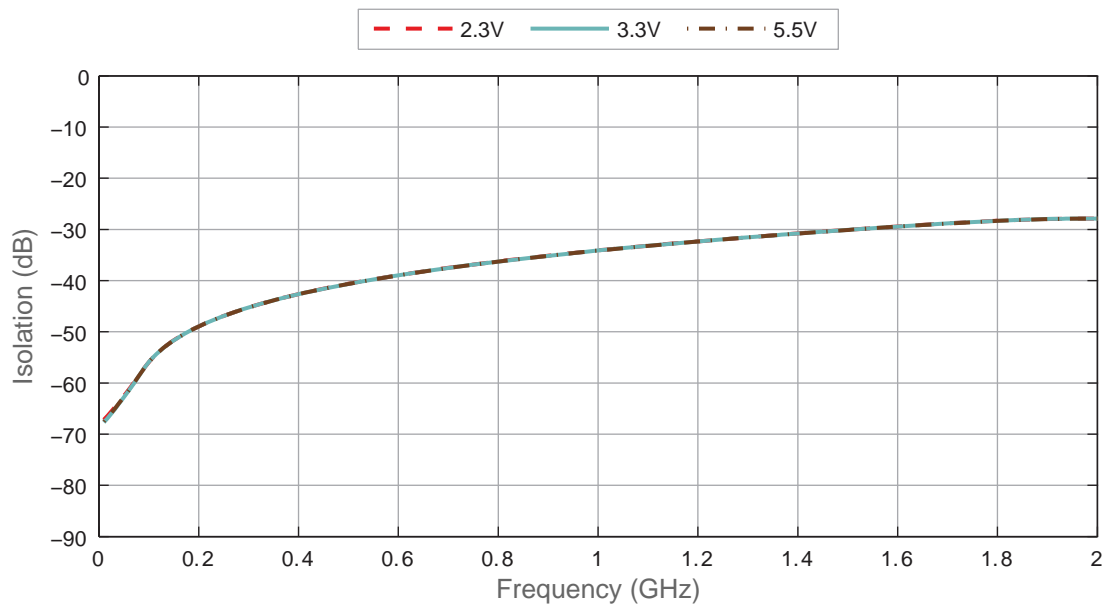
Figure 11 • Isolation vs. V_{DD} (RFC–RFX)
