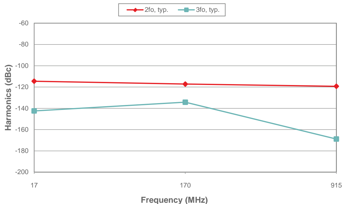
Figure 12 • Second and Third Harmonics ( P_{IN} = 65 dBmV)
