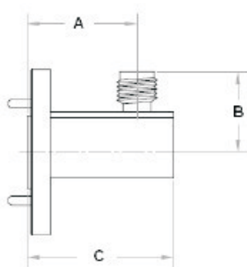
Figure 2 (Round Flange)
