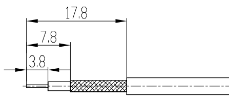
剥线尺寸 stripping dimension
