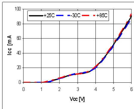
V-I Characteristics
