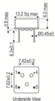
Underside View
