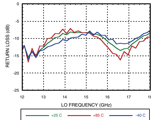
LO Return Loss vs. Temperature
