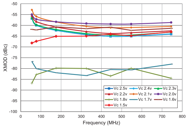
XMOD versus Frequency, 112 Channel 39dBmV Flat Input, Temp=+25°C
