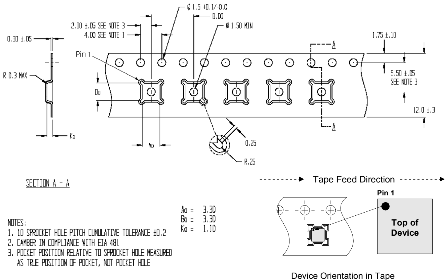
Figure 18. Marking Specifications
