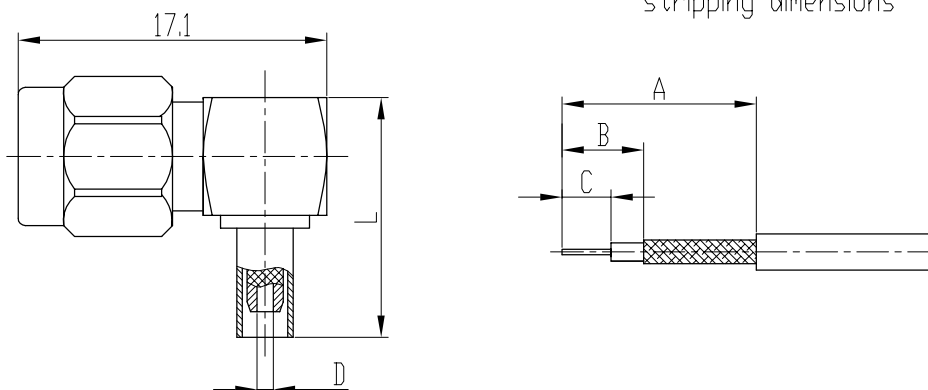
剥线尺寸 stripping dimensions
