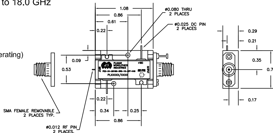
PE2 HOUSING WITHOUT CARRIER (SURFACE MOUNT)
