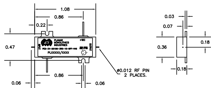
PE2 HOUSING WITHOUT CARRIER (SURFACE MOUNT)
