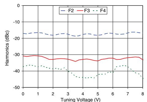
ROS-2700-1419+ Harmonics Level
