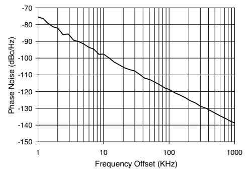
ROS-2700-1419+ Phase Noise
