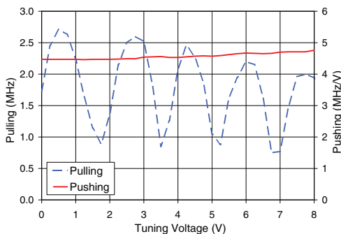
ROS-2700-1419+ Frequency Pulling & Pushing (Vcc ± 5%)
