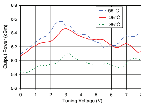
ROS-2700-1419+ Power Output
