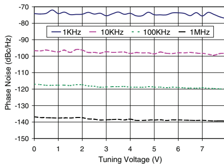
ROS-2700-1419+ Phase Noise Vs. Tuning Voltage
