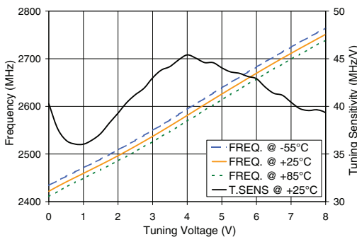
ROS-2700-1419+ Frequency and Tuning Sensitivity
