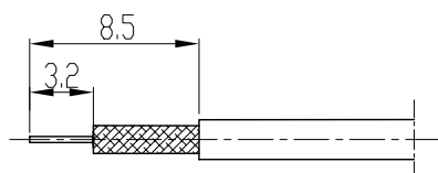
剥线尺寸 stripping dimension
