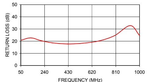
JTX-4-10T INPUT RETURN LOSS
