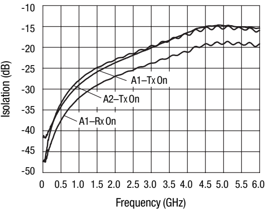
A2-Rx Isolation
