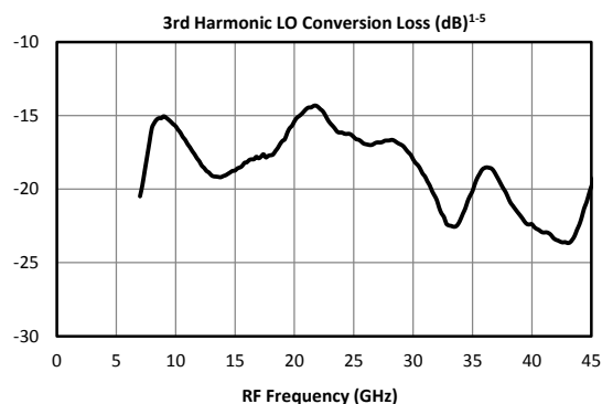
Typical Performance
