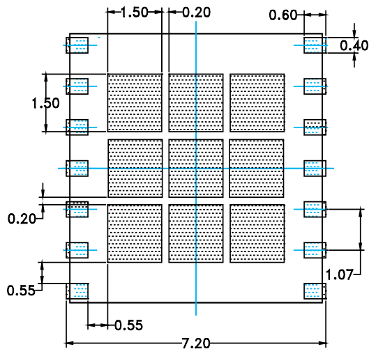
STENCIL APERTURE TOP (X-RAY) VIEW
