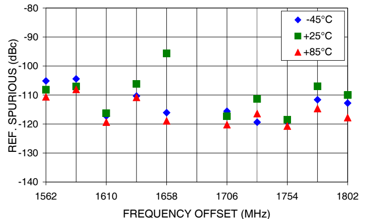
REFERENCE SPURIOUS Vs FREQ. OFFSET @ Fcar = 1682MHz
