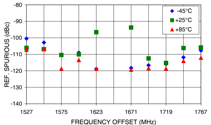
REFERENCE SPURIOUS Vs FREQ. OFFSET @ Fcar = 1646.5MHz
