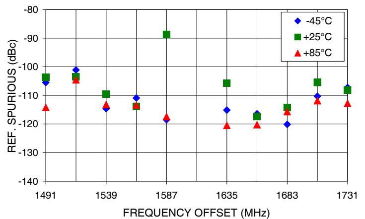
REFERENCE SPURIOUS Vs FREQ. OFFSET @ Fcar = 1611MHz
