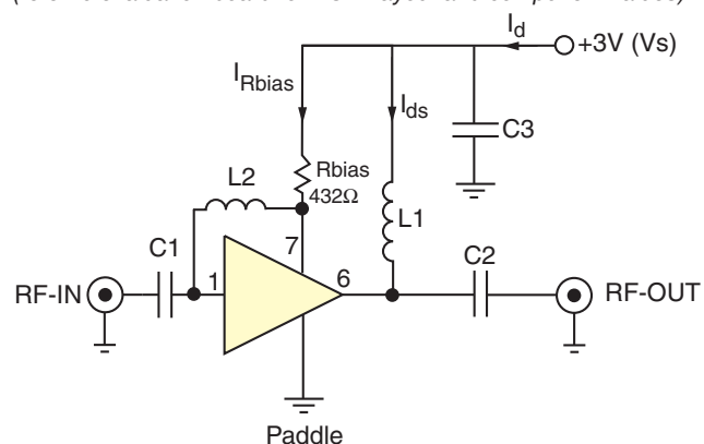
Fig 2. Recommended Application Circuit
