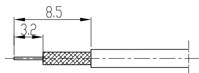
剥线尺寸 stripping dimensions
