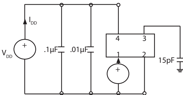
Fig 5: Test Circuit
