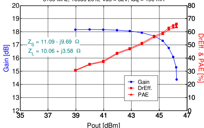
T1G4003532-FL Gain DrEff. and PAE vs. Pout
