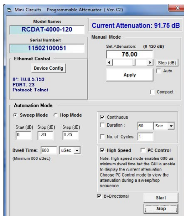
RCDAT GUI screen (Ethernet control, Sweep mode)
