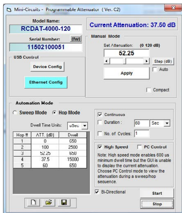
RCDAT GUI screen (USB control, Hop mode)
