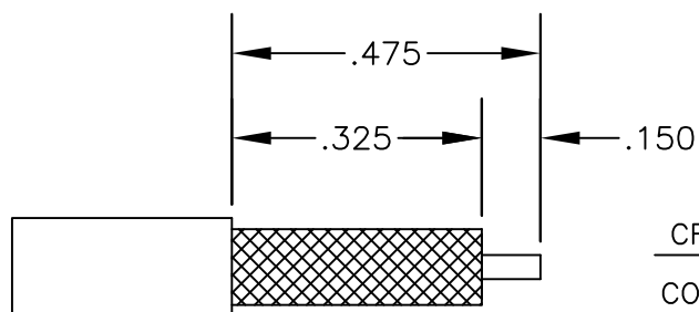
STRIPPING DIMENSIONS
