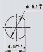
Mounting hole
