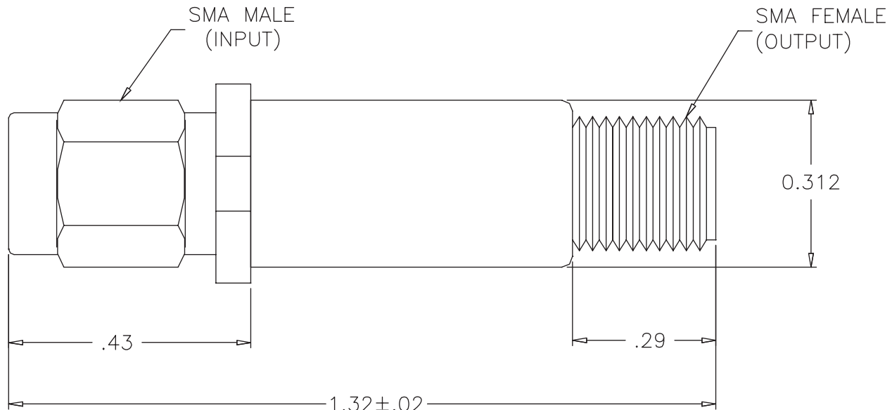
STANDARD CASE STYLE C3 (Optional Case Styles – C15, C32)
