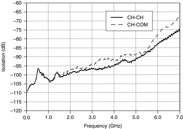
Figure 3. Typical Isolation
