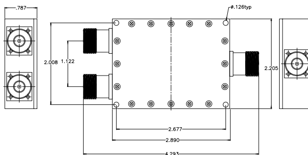
(800-2500 MHz 2-Way Power Divider with Isolation)
