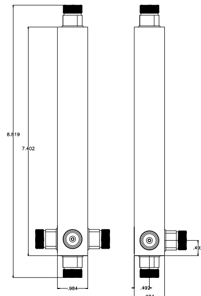
(800-2500 MHz Cavity Power Divider N)
