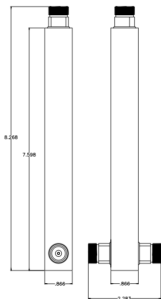
(800-2500 MHz Cavity Power Divider N)
