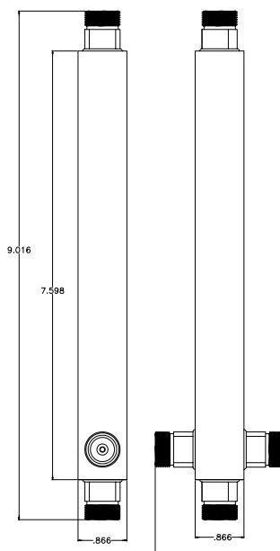
(800-2500 MHz Cavity Power Divider N)
