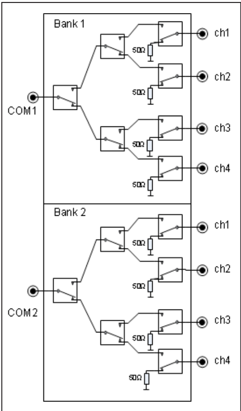
Figure 3. M9146A dual 1x4 RF switch multiplexer
