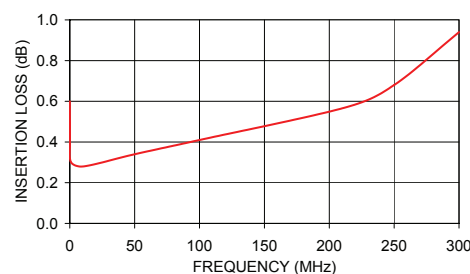
ADT4-6T INSERTION LOSS
