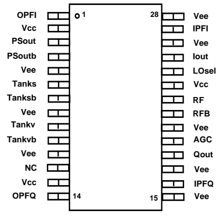
Figure 1 Pin connections
