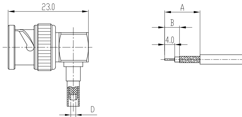
剥线尺寸 stripping dimensions
