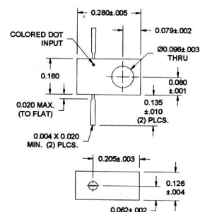
CASE STYLE M51
