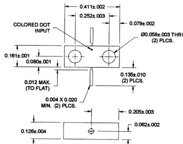
CASE STYLE M50
