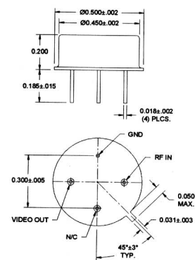
CASE STYLE M35
