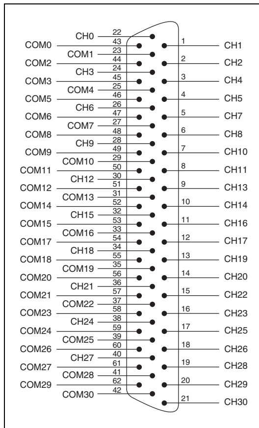
Figure 2. NI PXI-2568 Pinout
