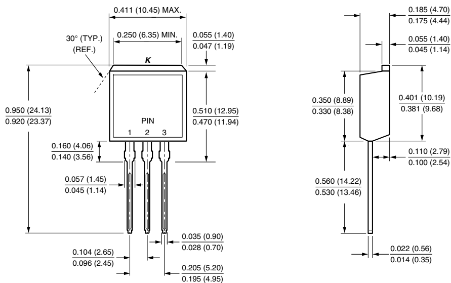
TO-262AA
