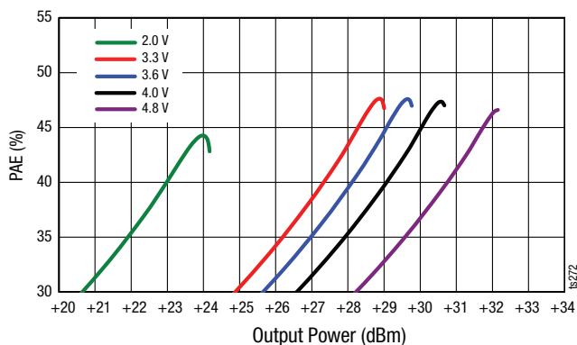
Figure 8. Typical PAE vs POUT & VCC, CW (VCC = 2.0 to 4.8 V) (including OMN and Antenna Filter Losses)
