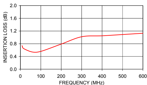
ADT2-1T-1P INSERTION LOSS
