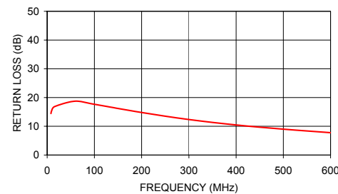
ADT2-1T-1P INPUT RETURN LOSS
