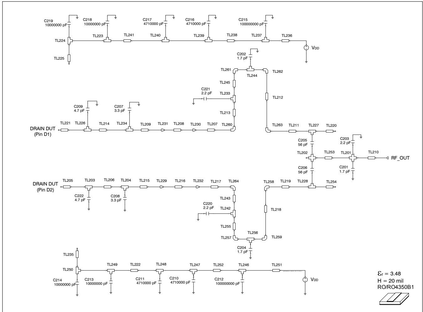
Reference circuit output schematic for f = 960 MHz
