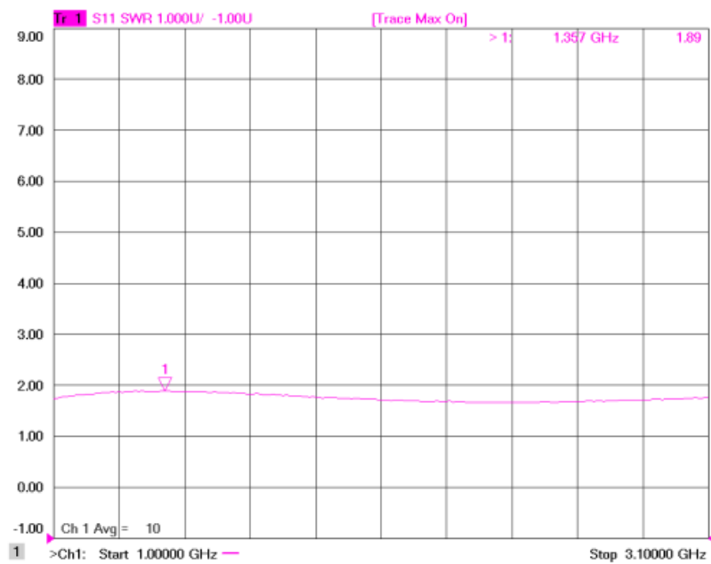
Figure 1-4: ERZ-LNA-0100-0310-30-2 Input Matching
