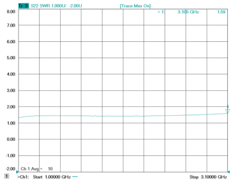
Figure 1-5: ERZ-LNA-0100-0310-30-2 Output Matching
