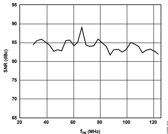
Figure 8. Single Tone SNR vs. Input Frequency ( f_{\text{IN}} )
