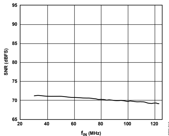
Figure 7. Single Tone SNR vs. Input Frequency ( f_{\text{IN}} )
