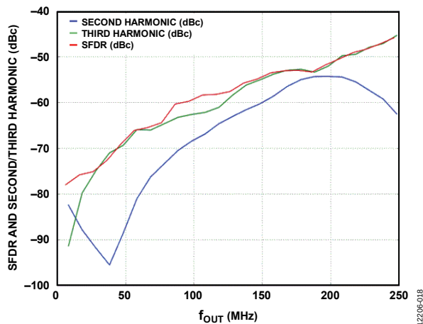
Figure 13. SFDR, 2 nd and 3 rd Harmonics vs. f_{OUT} , Maximum I_{OUTS} (DAC Gain)
