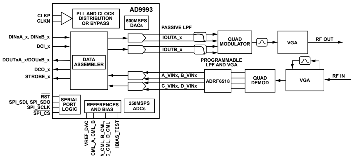
Figure 32. Radio Signal Chain Example
